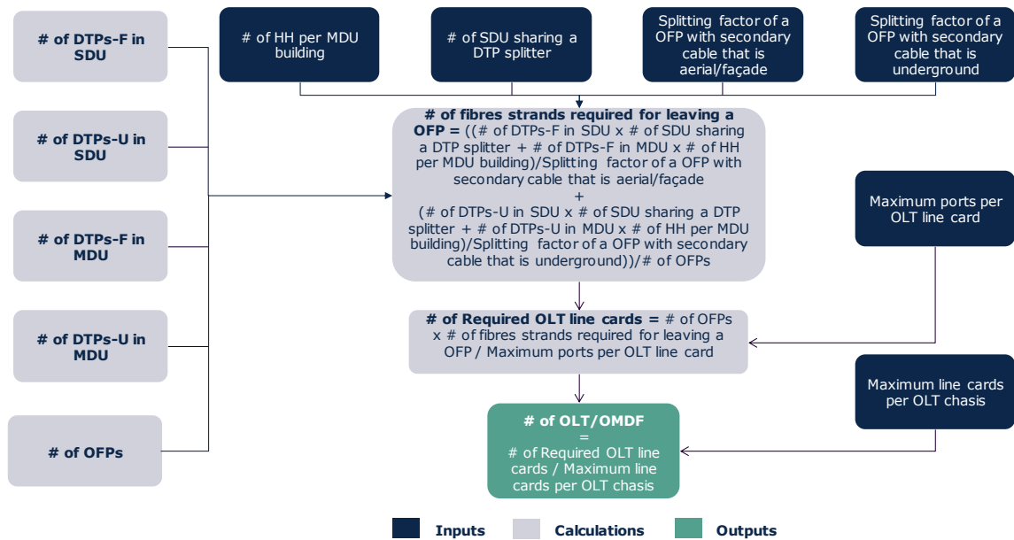
Exhibit 6.12: Algorithm for calculating the number of OLTs and OMDFs [Source: Axon Consulting]
