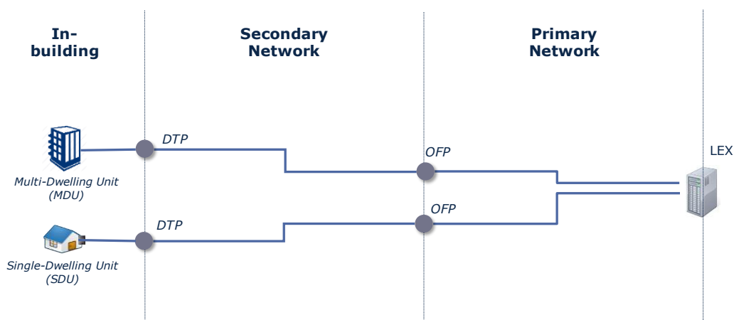
Exhibit 6.1: Architecture of the modelled Access Network [Source: Axon Consulting]
