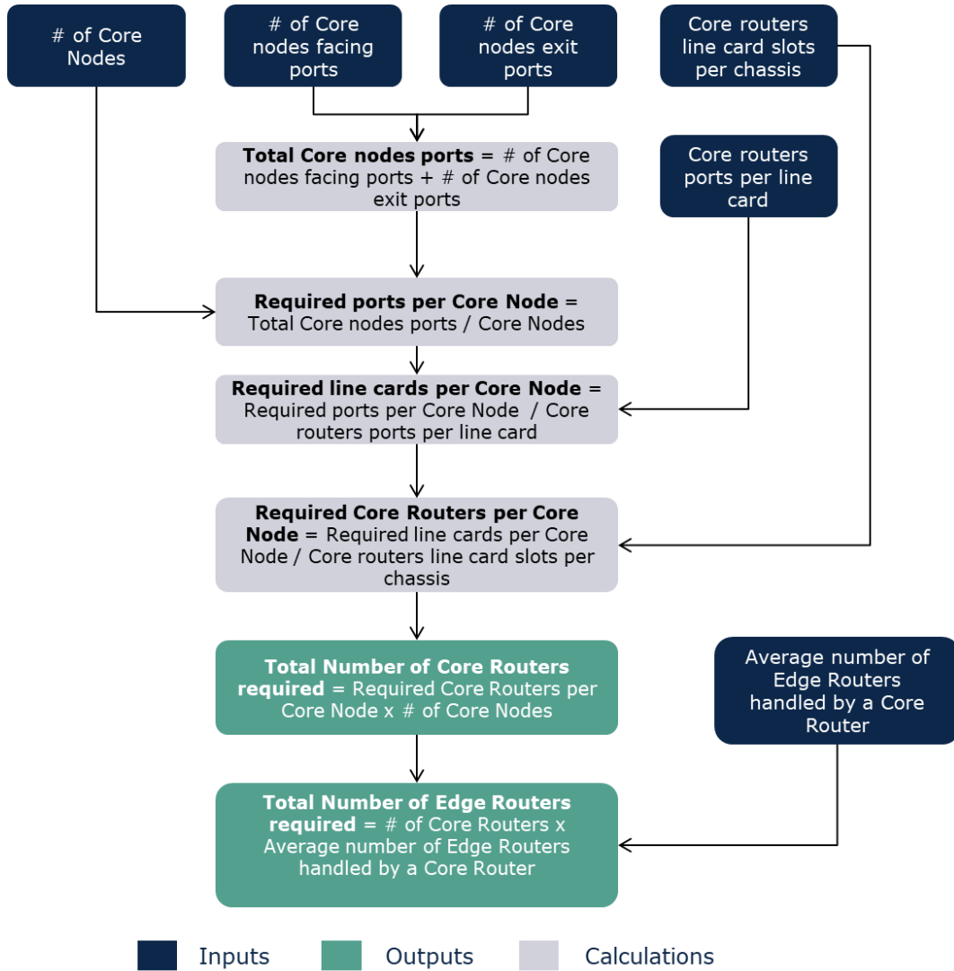
Exhibit 6.17: Algorithm employed to calculate the number of Core Routers required [Source: Axon Consulting]
