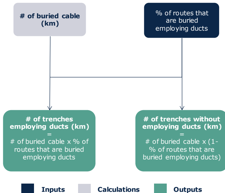
Exhibit 6.9: Algorithm for calculating the kilometres of trenches employing or not ducts in the access network [Source: Axon Consulting]
